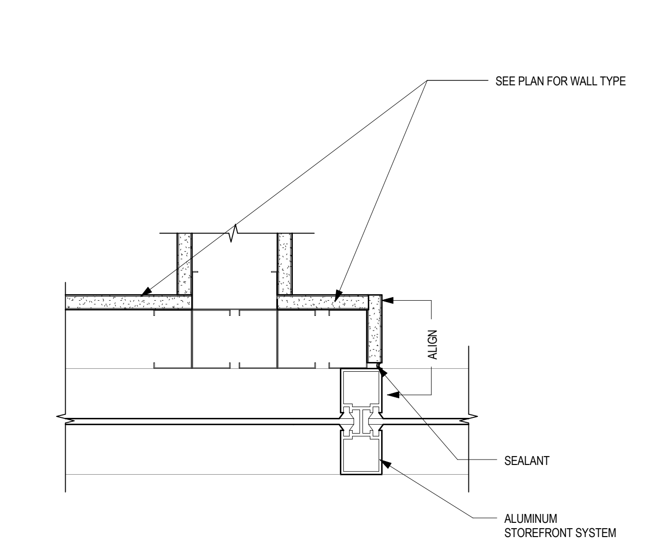
9 PLAN DETAIL AT WALL TO STOREFRONT 3" = 1'-0"
