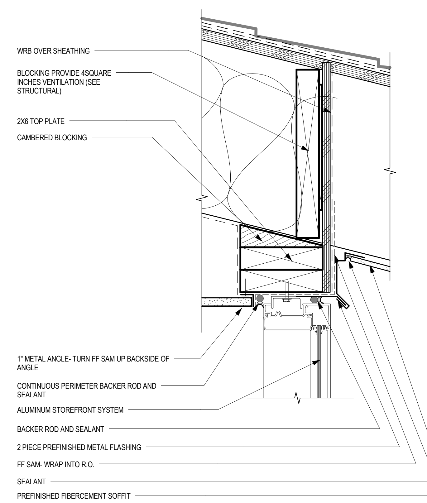
12 SF HEAD @ GLULAM BEAM 3" = 1'-0"
