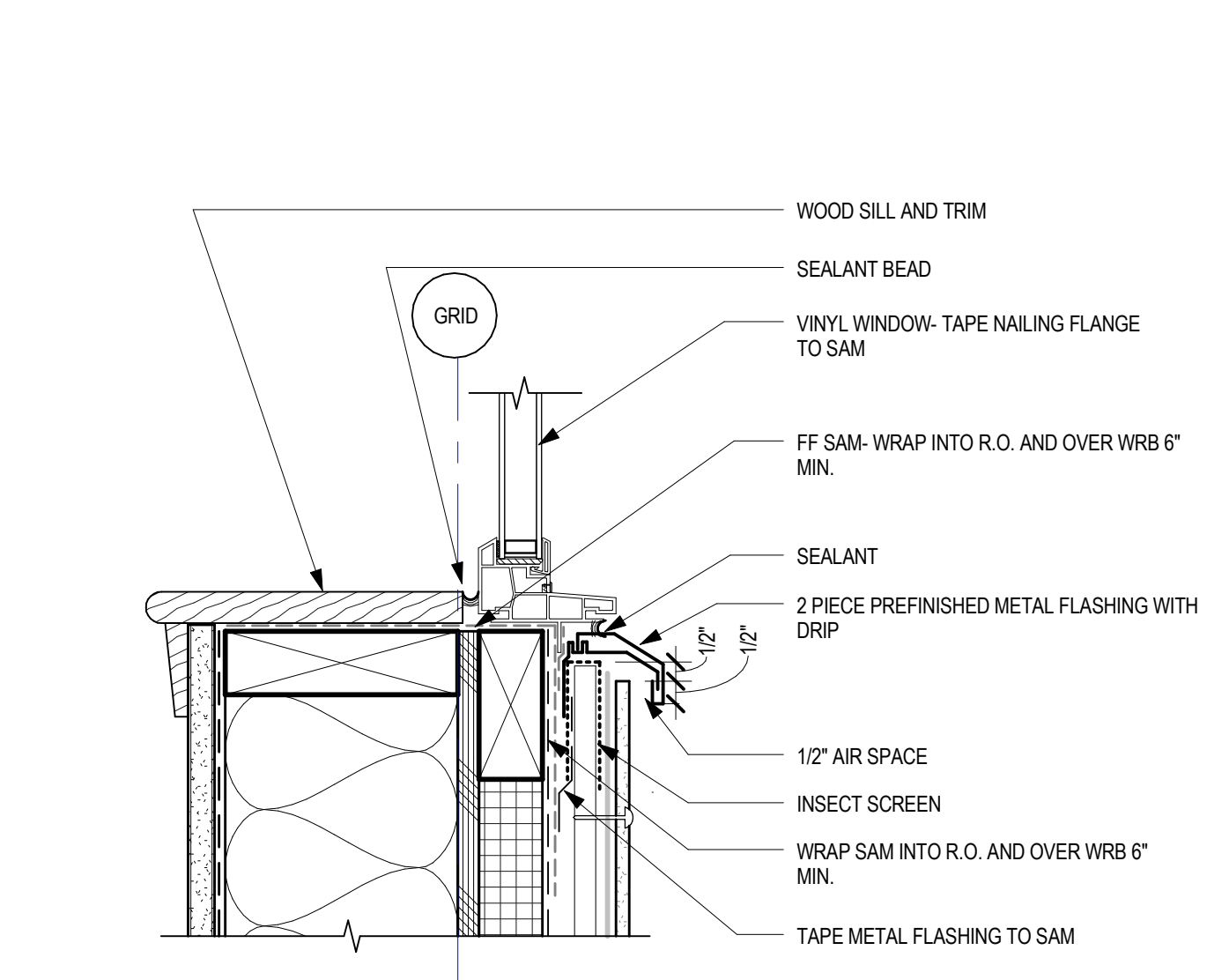
2 WINDOW JAMB1 3" = 1'-0"
