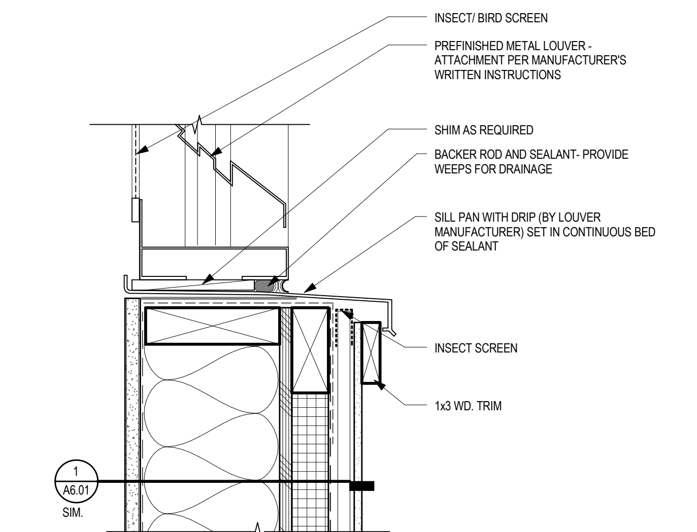
13 LOUVER SILL1 3" = 1'-0"
