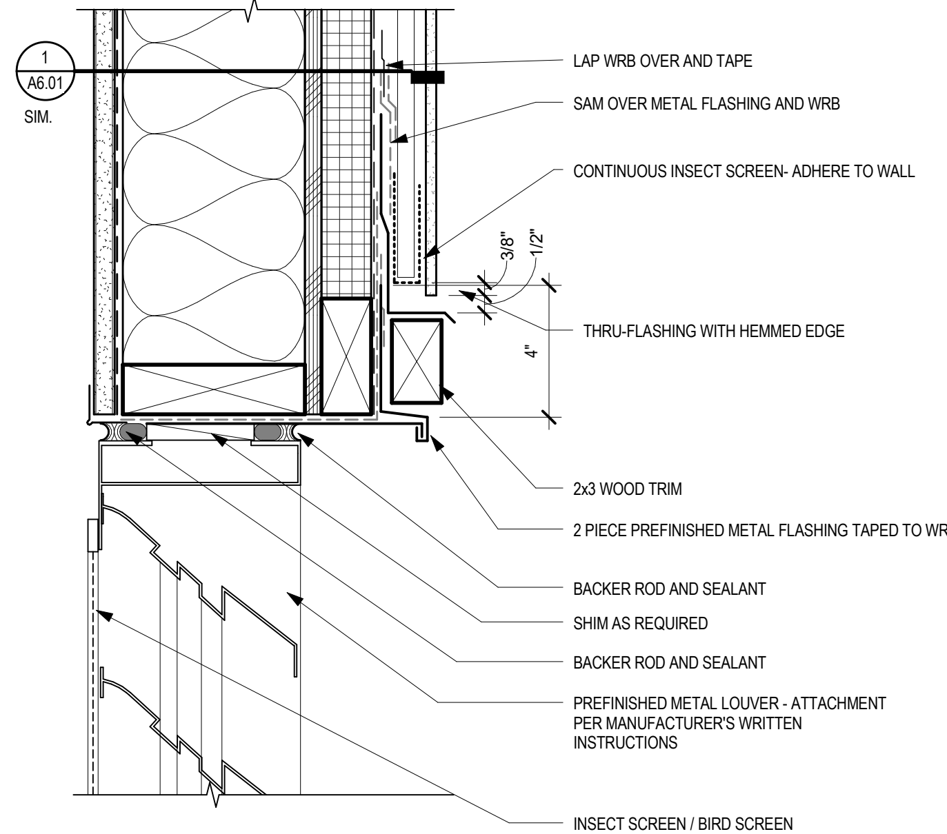
15 LOUVER HEAD1 3" = 1'-0"
