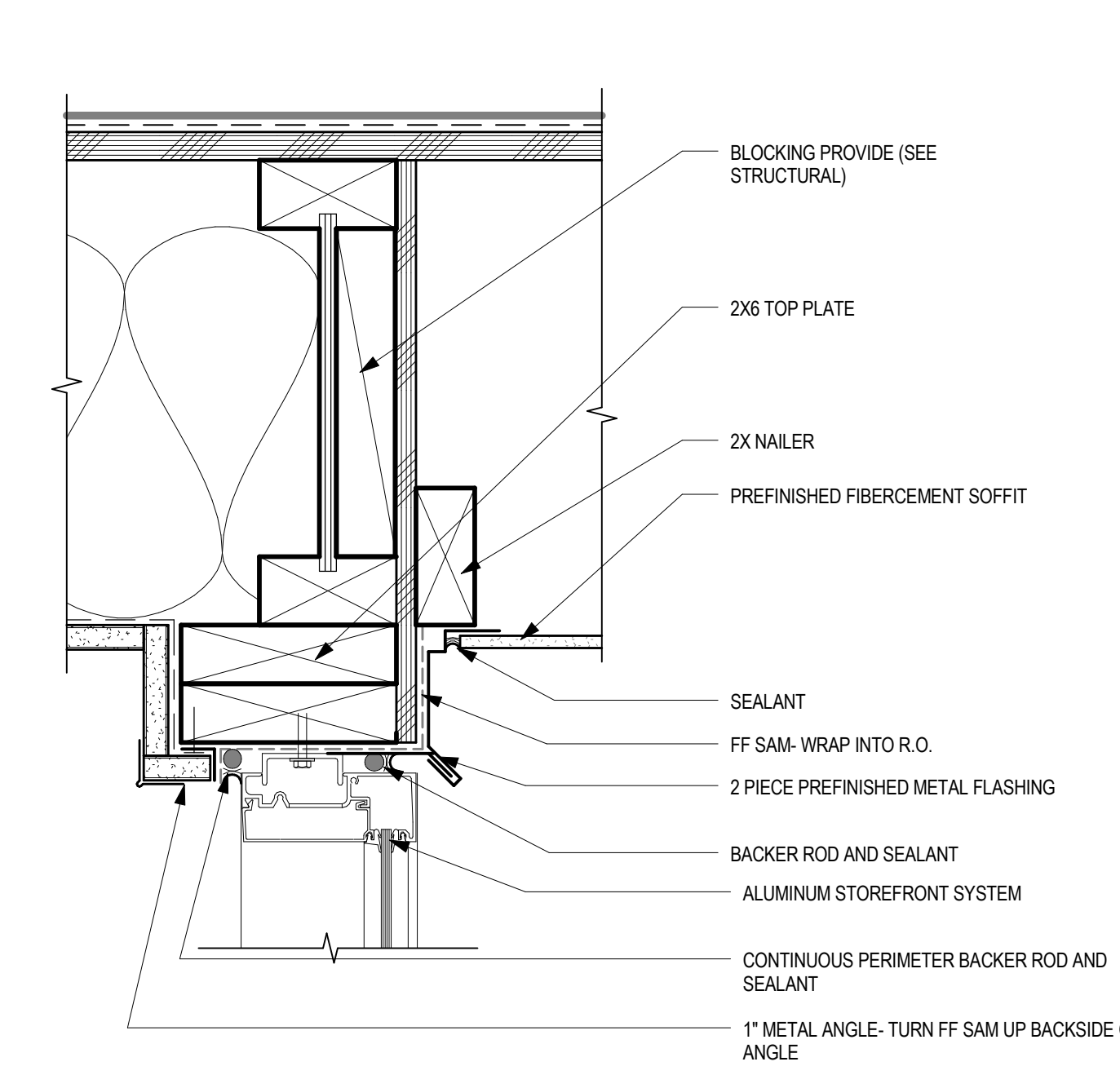
8 SF HEAD AT RAKE1 3" = 1'-0"
