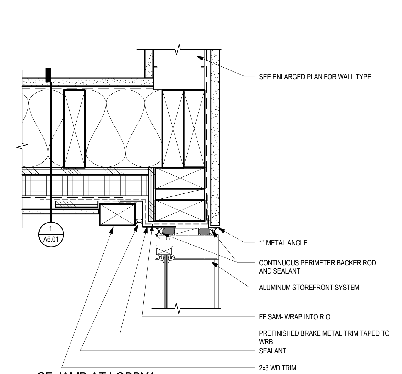
10 SF JAMB AT LOBBY1 3" = 1'-0"
