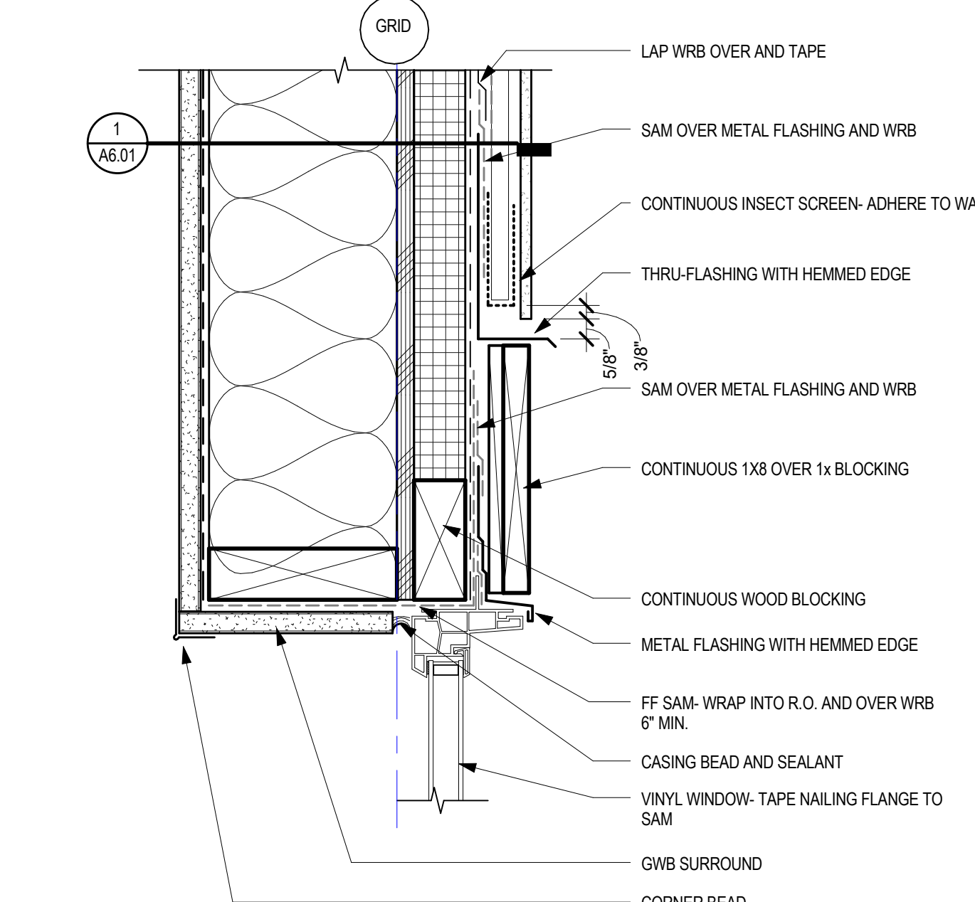
3 WINDOW HEAD1 3" = 1'-0"
