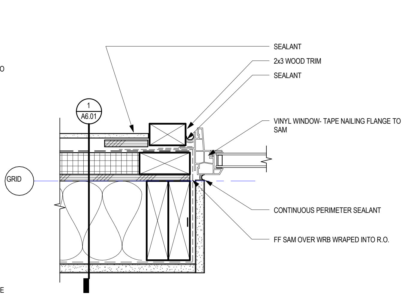
3 WINDOW HEAD1 3" = 1'-0"
