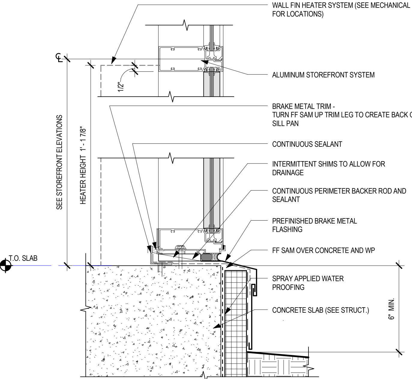
5 SF SILL AT SLAB 3" = 1'-0"
